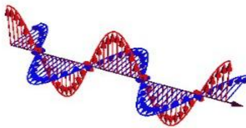
Electromagnetic wave
