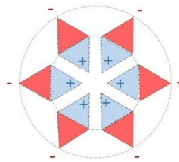
Particle of Light
