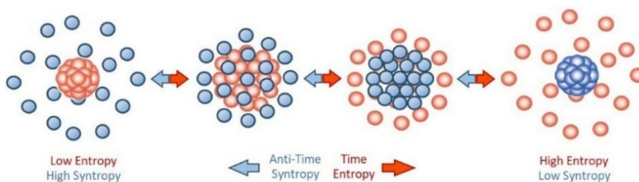
Time & Anti-time - Entropy and symmetry
