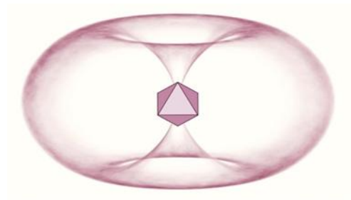
Origin of subatomic particles in Space and Negative space
