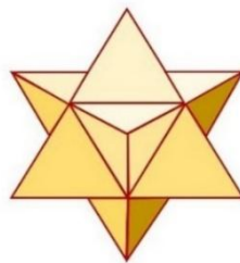
Photon shell (star tetrahedron)
