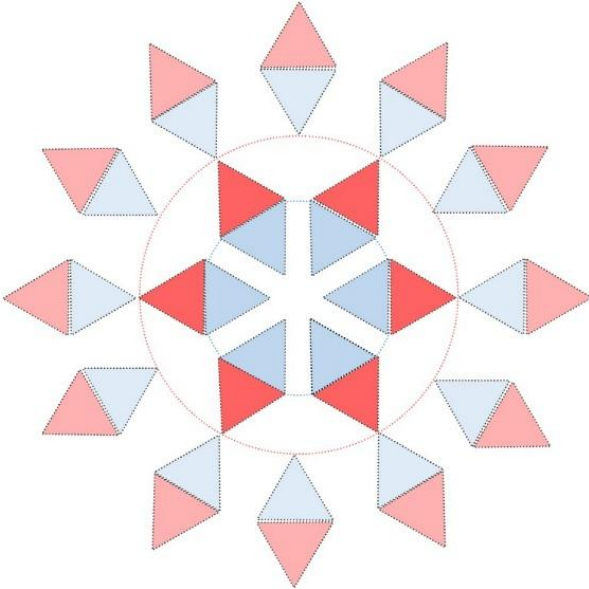
Wavelets of Light
