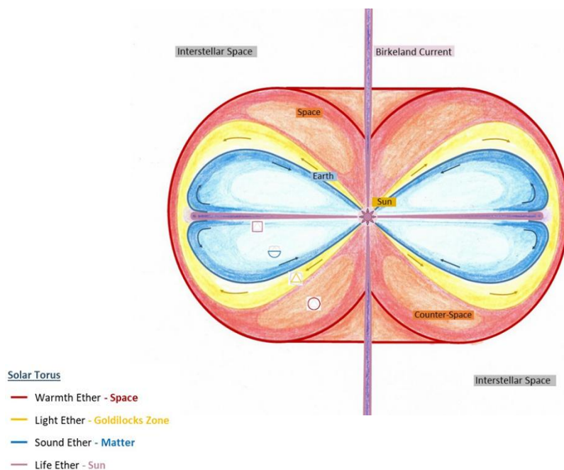
Figure B.2 – Solar Torus Energy Fields
