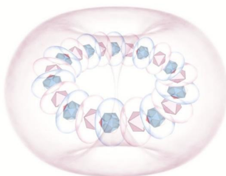
Figure 4.1 - The Atomic nucleus ring ( ^{10}\text{Ne} )
