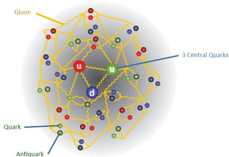
Figure 3.1 - Proton, quark-gluon tangle - Image DESY
