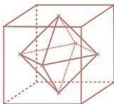
Figure 2.7 - Cube dual, the octahedron
