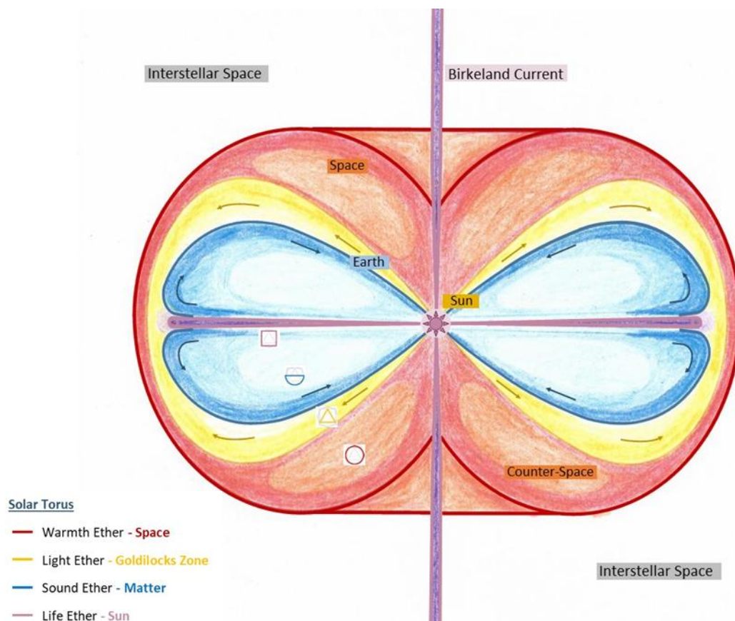
Figure B.2 – Solar Torus Energy Fields
