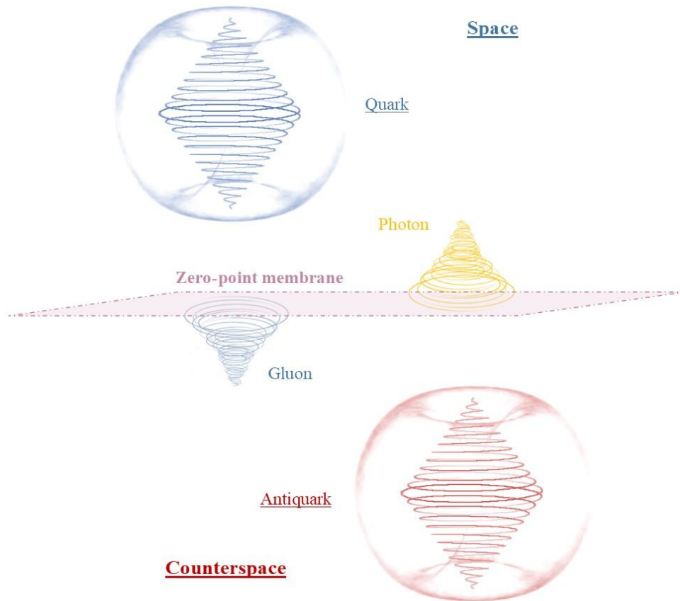
Figure 2.5 - The zero-point matrix
