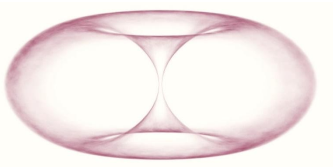
Figure 2.1 - The Universal torus
