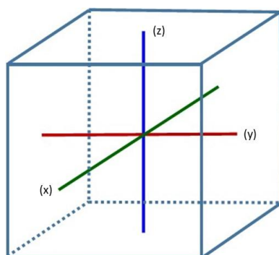
Figure 2.6 - Cube - The three dimensions
