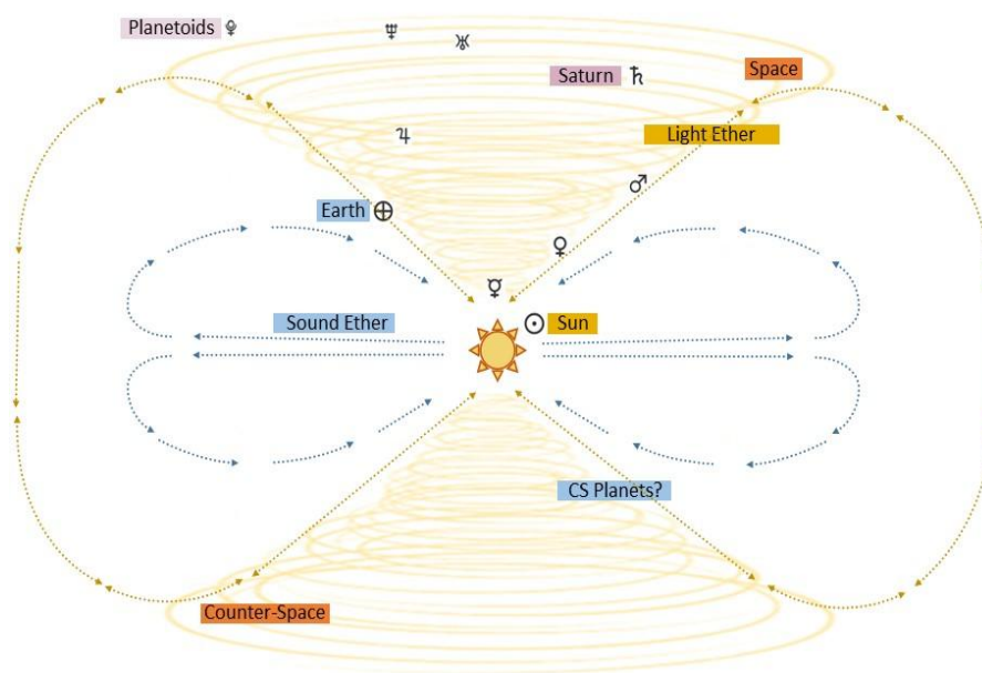
Figure B.1. The Solar Torus Vortexes
