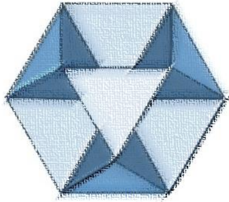
Figure 2.8 – Octahemioctahedron – Gluon Equilibrium
