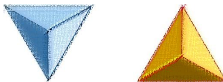
Figure 2.4 - The Gluon & the Photon
